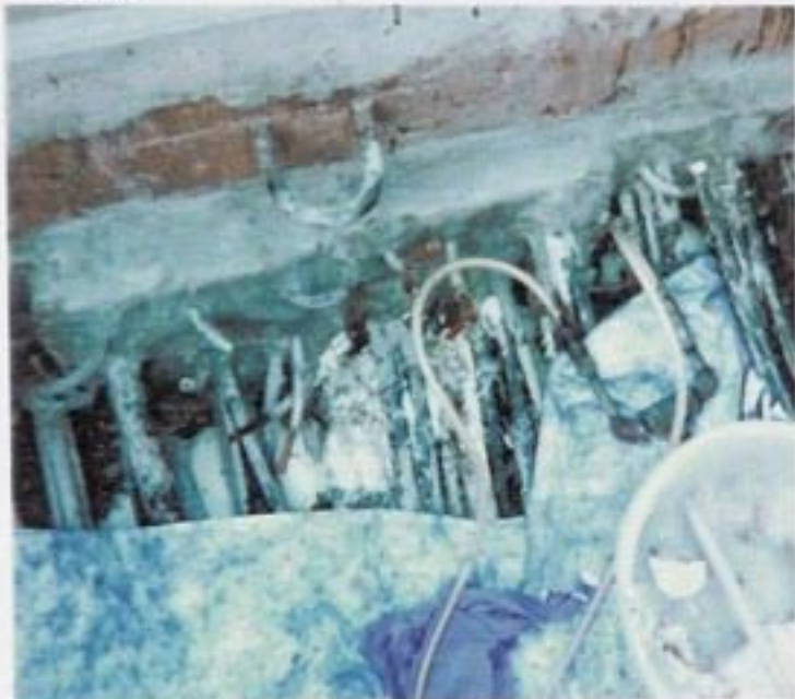
Close up view showing FX-III Jet Set pumped into conduits packed with jute rope.
