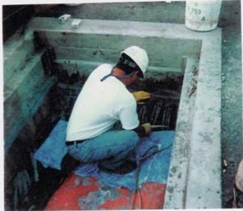
The ducts are sealed using FX-III Jet Set and plain jute rope.
